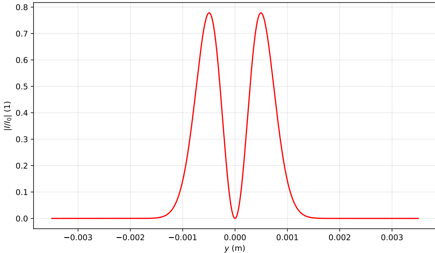
Intensity profile I(x=0, y, z=0.080)/I_0 , \text{Pin}=3.0\text{Pcr} , artificial time
